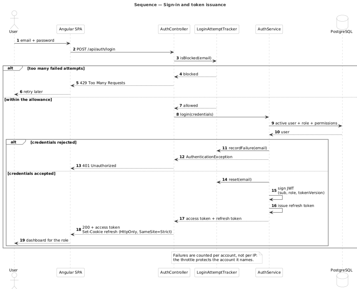
Figure 4.2: Sequence diagram of the “Authenticate” use case
