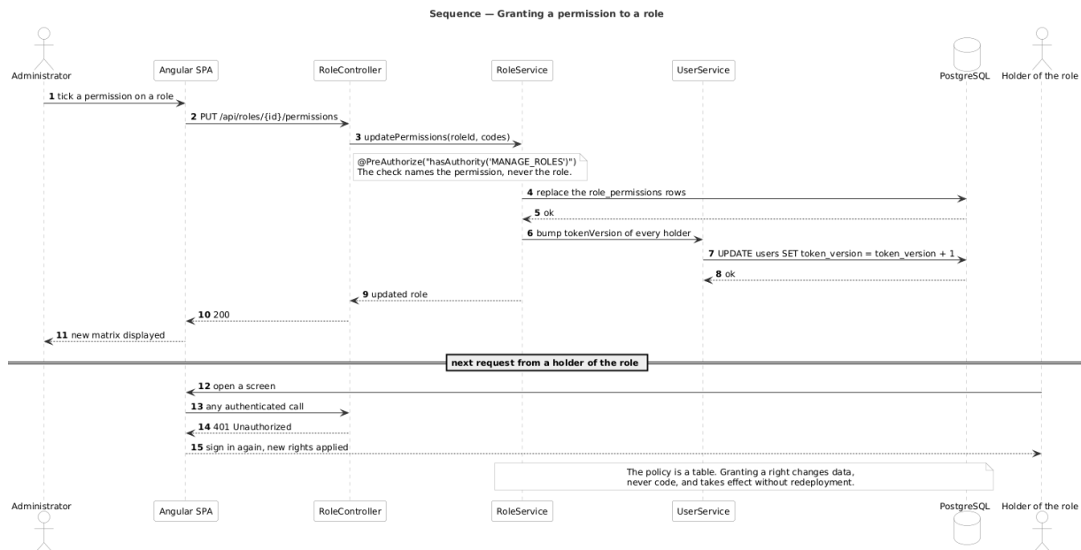
Figure 4.9: Sequence diagram of the “Grant a permission to a role” use case
