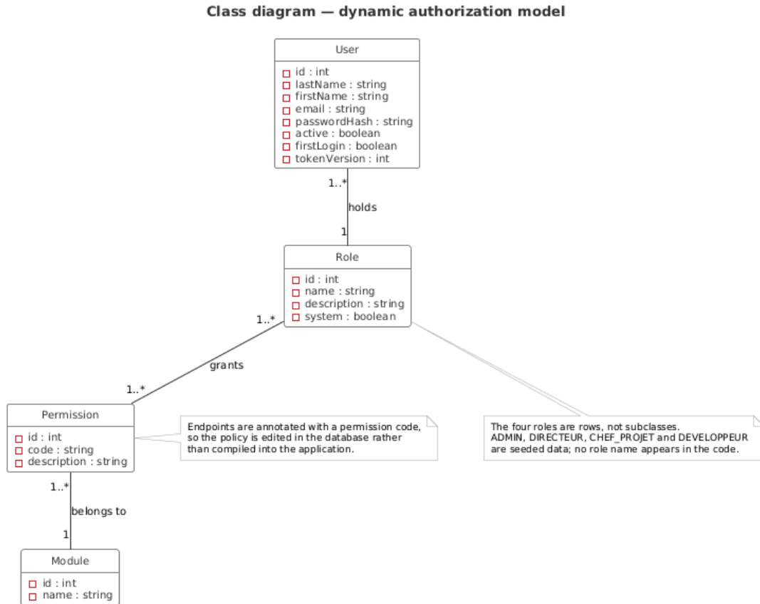
Figure 4.8: Class diagram of the authorization model
